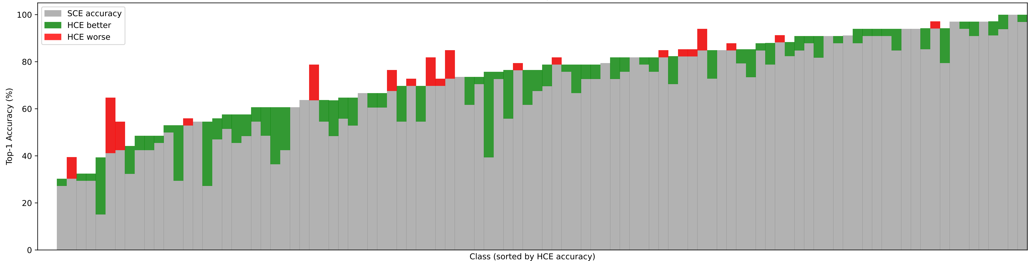
ResNet-18 — Per-leaf-class accuracy: SCE vs HCE (FGVC Aircraft)
